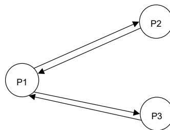
Figure 4.2: Deadlock in AND Request Model
