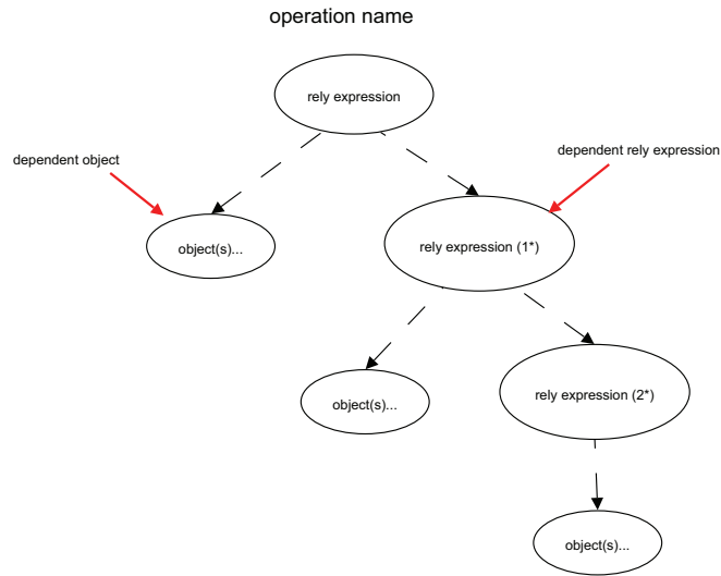
Figure 5.4: Example of Rely Diagram Structure with Nested Rely Expressions
