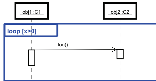
Figure 2.3: Example of Using Interaction Operator loop
